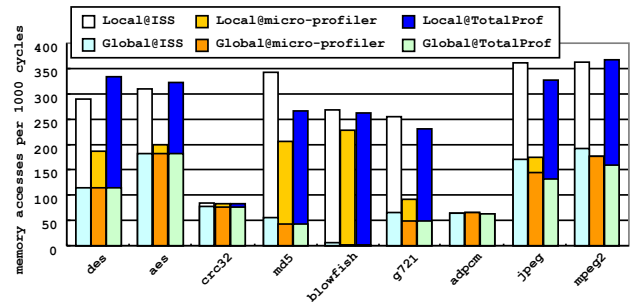
(b) Global and local memory accesses
