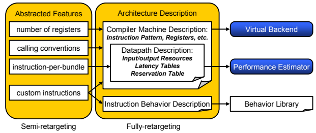
Figure 4: Retargeting TotalProf
